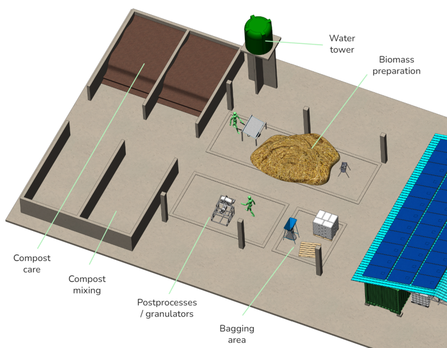
3D Design of the bio-fertilizer production facility
